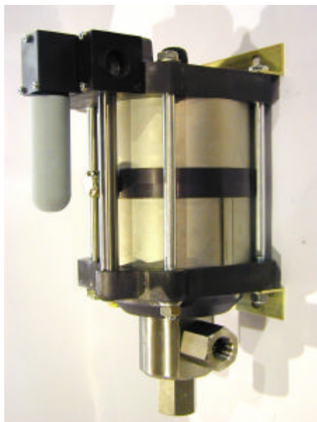
G25-2(L) single acting, double air drive head (Standard= Bottom inlet)
