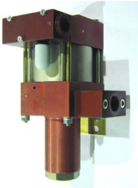
M8(L) single acting, single air drive head (Standard= Bottom inlet)
