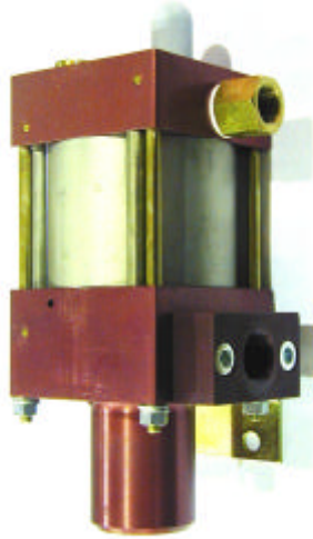
MO4 single acting, single air drive head (Standard= Bottom inlet)
